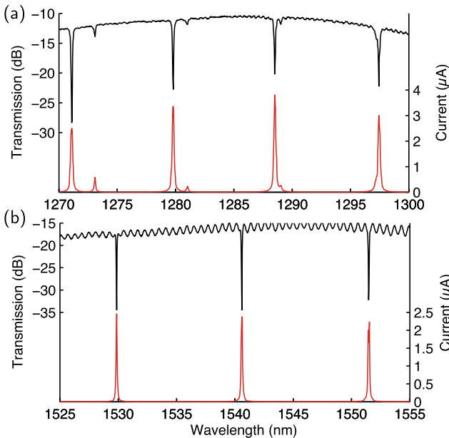
Fig. 2. Fiber-fiber transmission and photocurrent spectra through devices operating near (a) 1280 and (b) 1550 nm, with -1 V bias applied and approximately 80 \mu W optical power propagating to the device in the input fiber before the input grating coupler.
